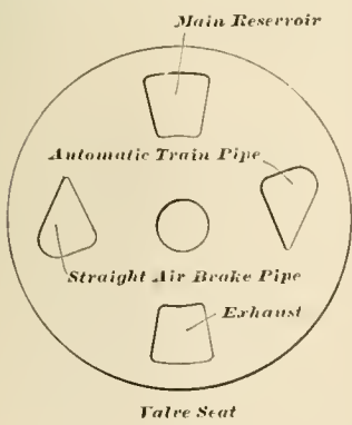
PLAN VIEW OF VALVE SEAT.
